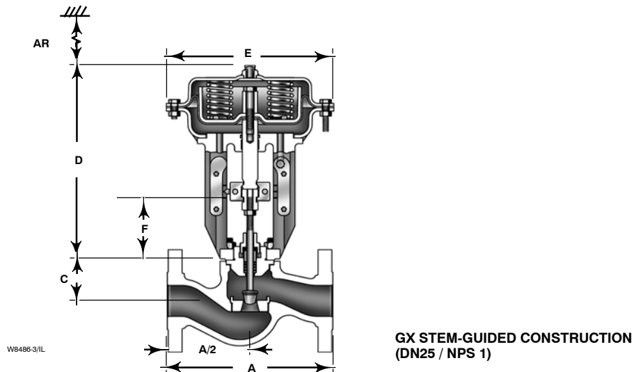
Figure 18. Fisher GX Dimensions (also see table 19)
