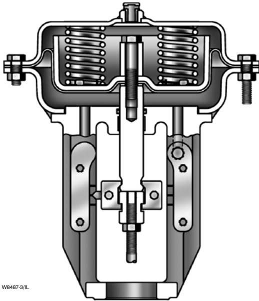
Figure 15. Fisher GX Actuator
