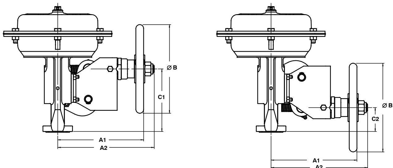
Figure 23. Fisher GX with Handwheel Dimensions (also see table 21)
