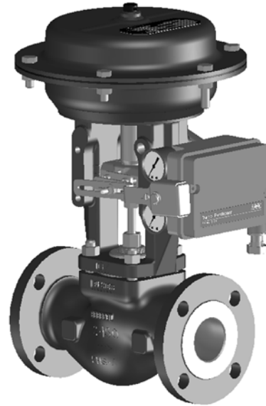
Figure 20. Fisher GX Valve with 3660 or 3661 Positioner, NAMUR Mounting (IEC 60534-6-1)
