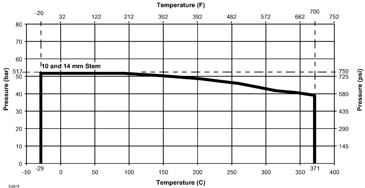
Figure 17. Bellows Pressure - Temperature Ratings
