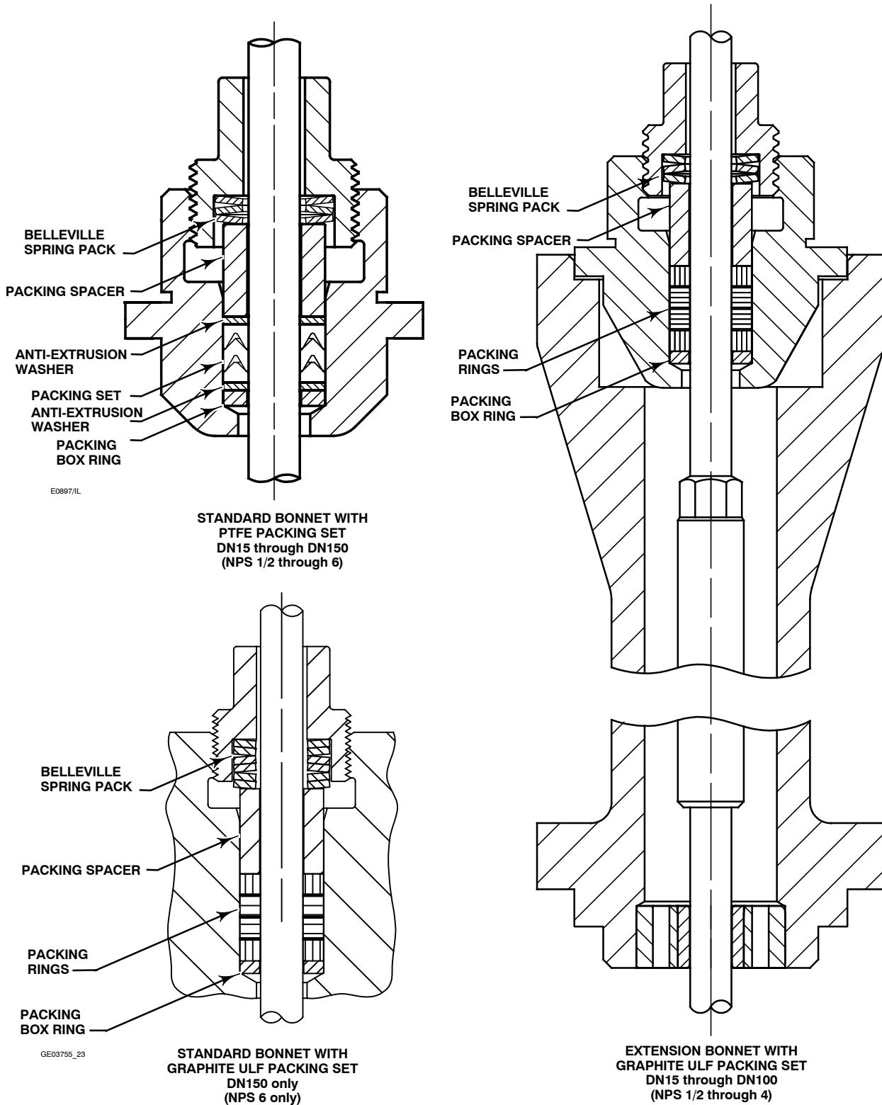
Figure 12. Fisher GX Packing
