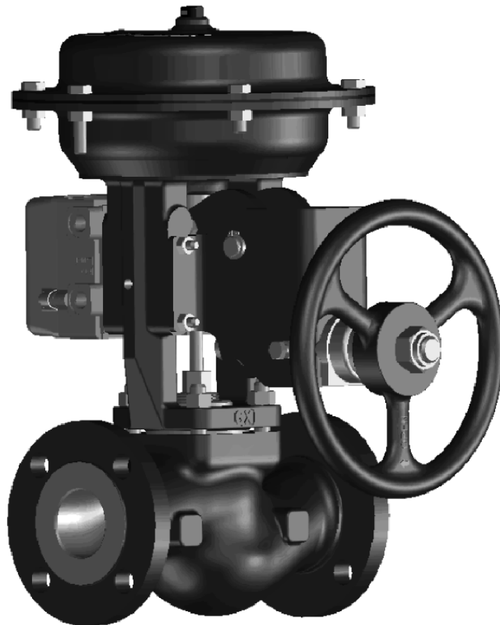
Figure 22. Fisher GX Control Valve and Actuator System with Manual Handwheel
