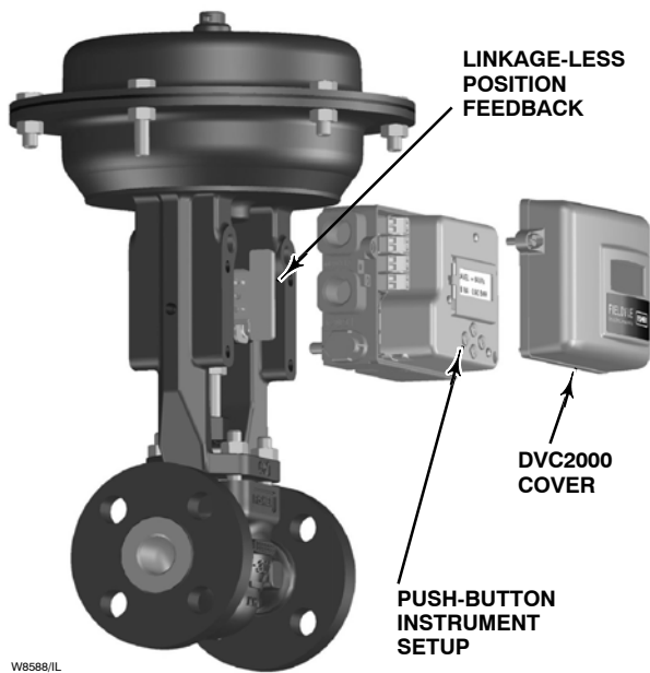
Figure 3. Fisher GX and DVC2000 Digital Valve Controller
